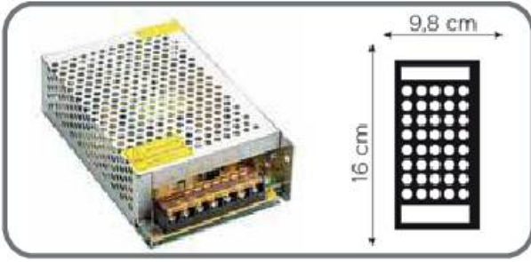
10A 120W POWER SUPPLY TRAFÖ
