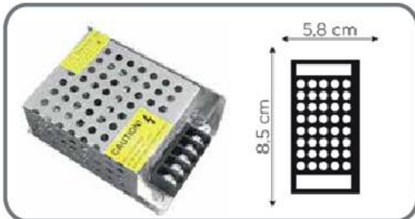
3.33A 36W POWER SUPPLY TRAFÖ
