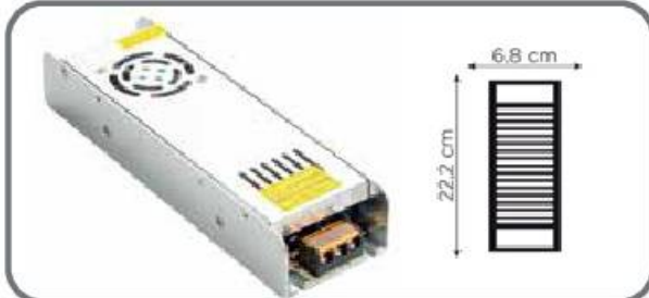
30A 360W SLIM POWER SUPPLY TRAFÖ
